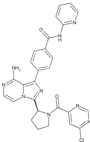
(S)-4-(8-amino-3-(1-(6-clopyrimidin-4-cacbonyl)pyrrolidin-2-yl)imidazo[1,5-a]pyrazin-1-yl)-N-(pyridin-2-yl)benzamidit
