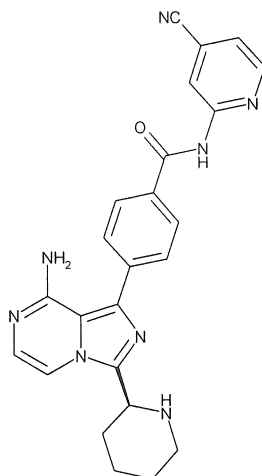
(S)-4-(8-amino-3-(piperidin-2-yl)imidazo[1,5-a]pyrazin-1-yl)-N-(4-cyanopyridin-2-yl)benzamidit
