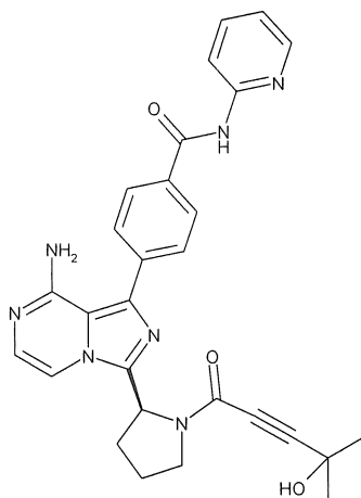
(S)-4-(8-amino-3-(1-(4-hydroxy-4-methylpent-2-ynoyl)pyrrolidin-2-yl)imidazo[1,5-a]pyrazin-1-yl)-N-(pyridin-2-yl)benzamidit
