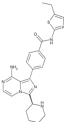
(S)-4-(8-amino-3-(piperidin-2-yl)imidazo[1,5-a]pyrazin-1-yl)-N-(5-ethylthiazol-2-yl)benzamid
